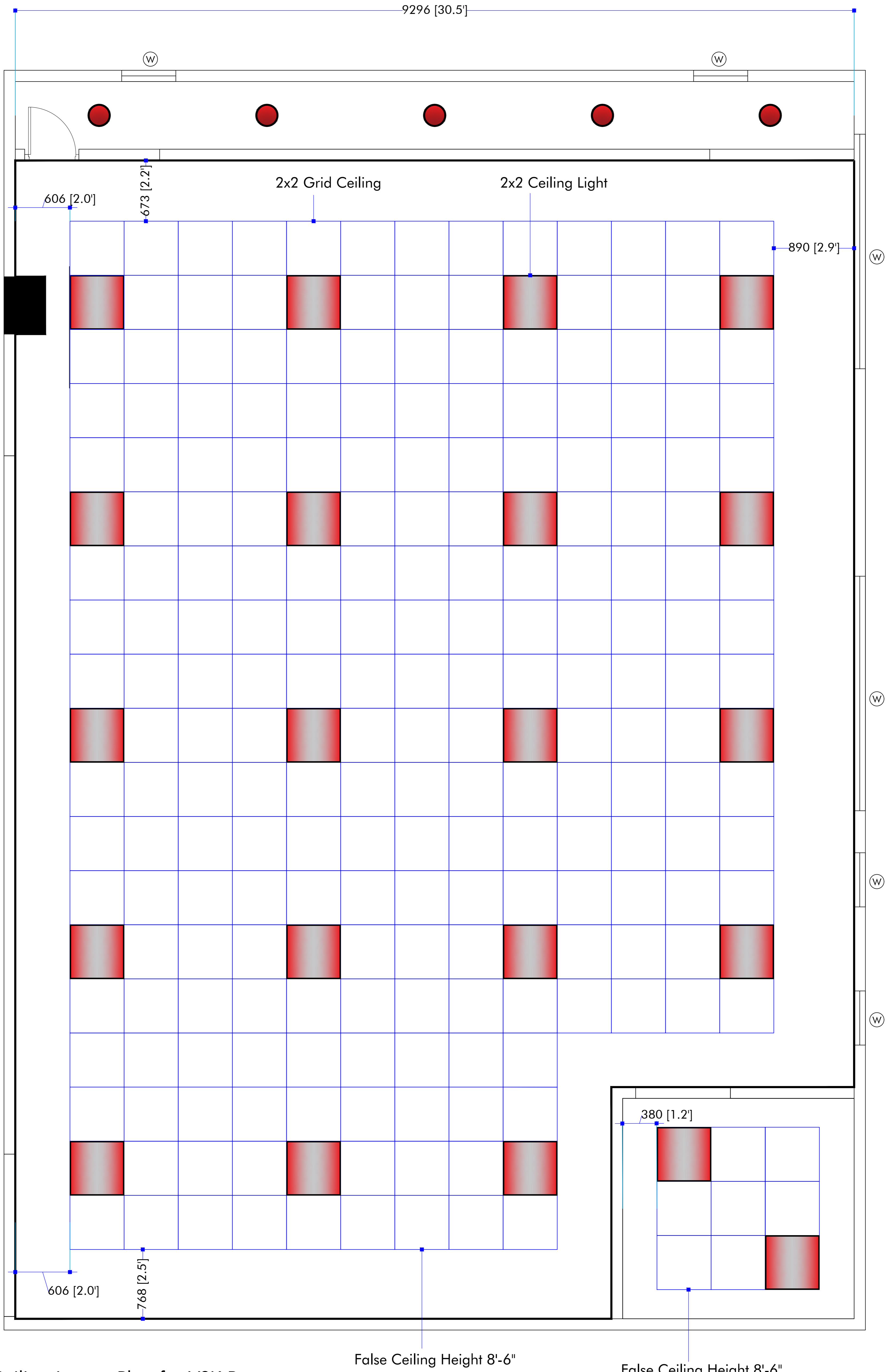
Proposed Ceiling Layout Plan for VSK Room
